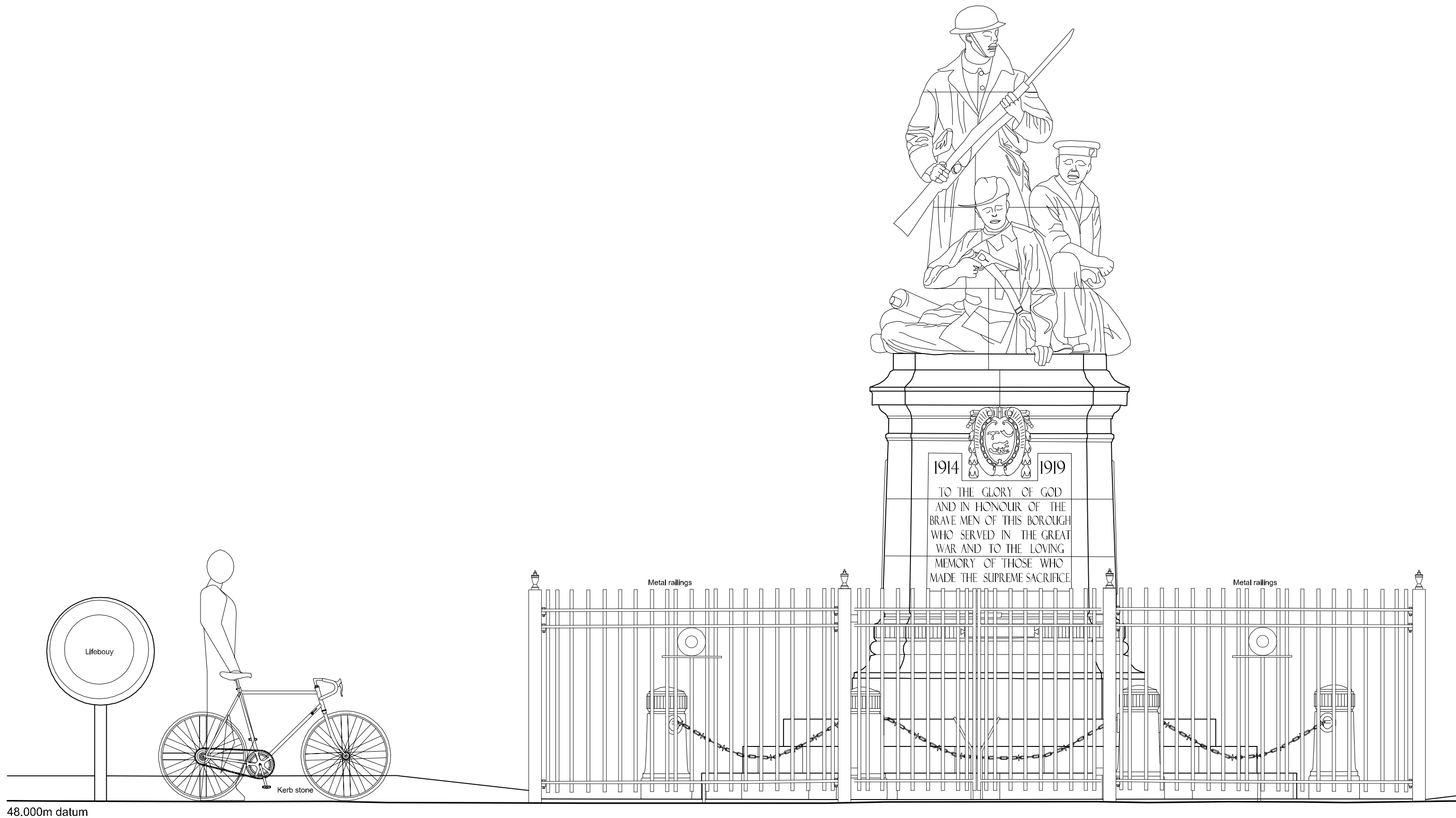
FRONT ELEVATION SCALE 1:25
